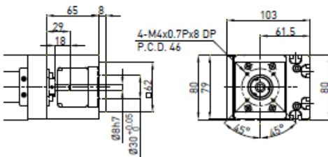
Motor Adaptor Flange F2
