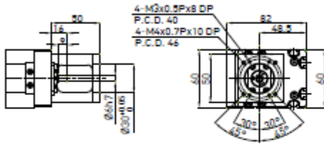
Motor Adaptor Flange F0
