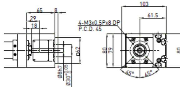
Motor Adaptor Flange F3
