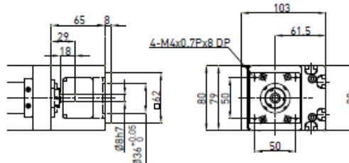
Motor Adaptor Flange F5
